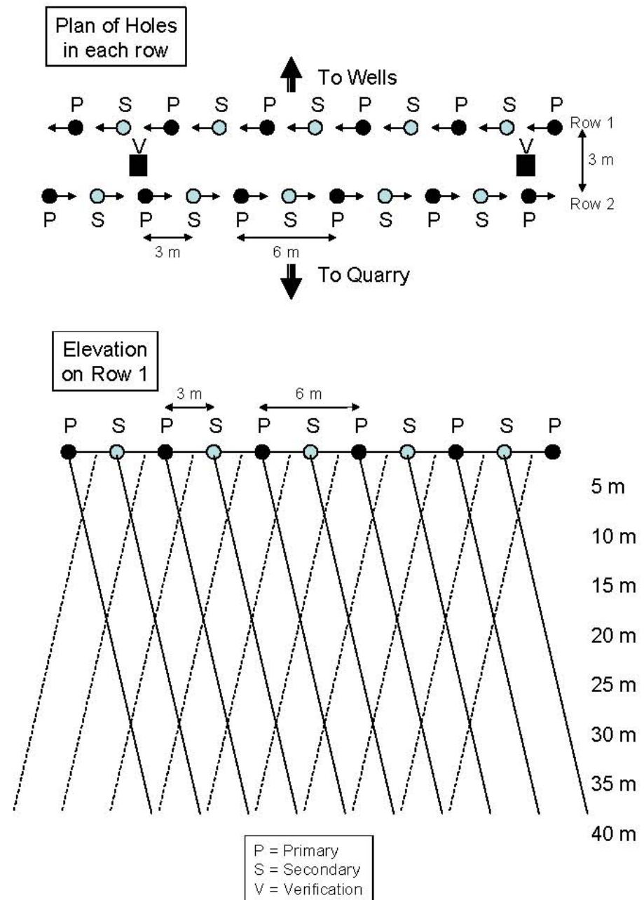
Sketch 1. Foreseen geometry of the two-row grout curtain.
